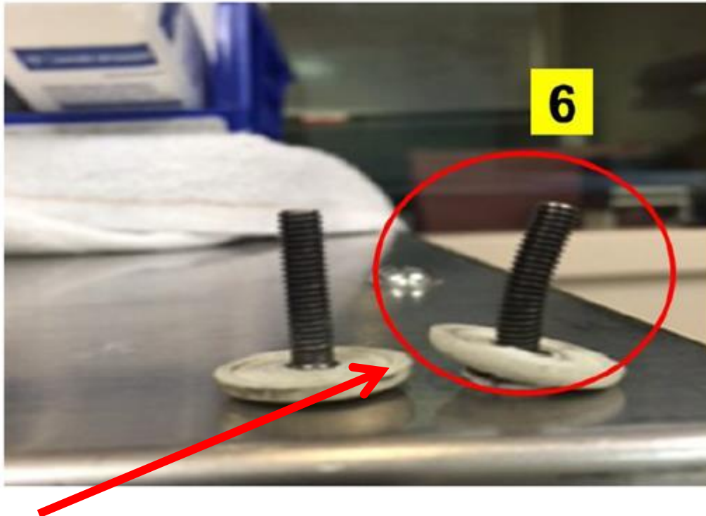
6. Bent screw found, preventing table from full range of horizontal motion
