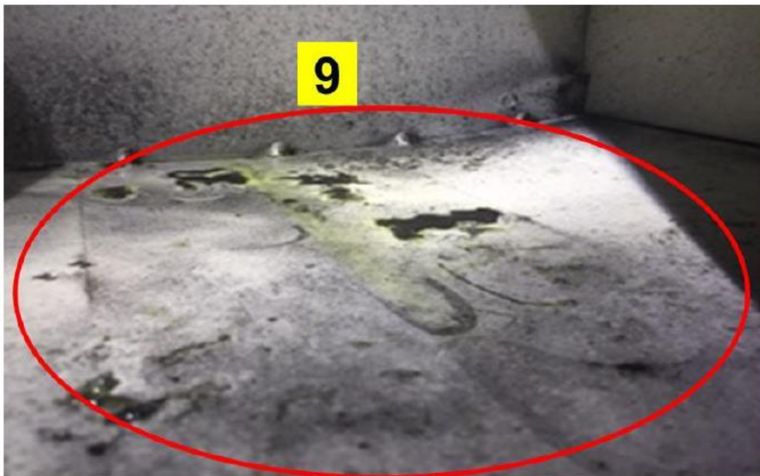
9. Oil and debris identified in back corners of gantry
