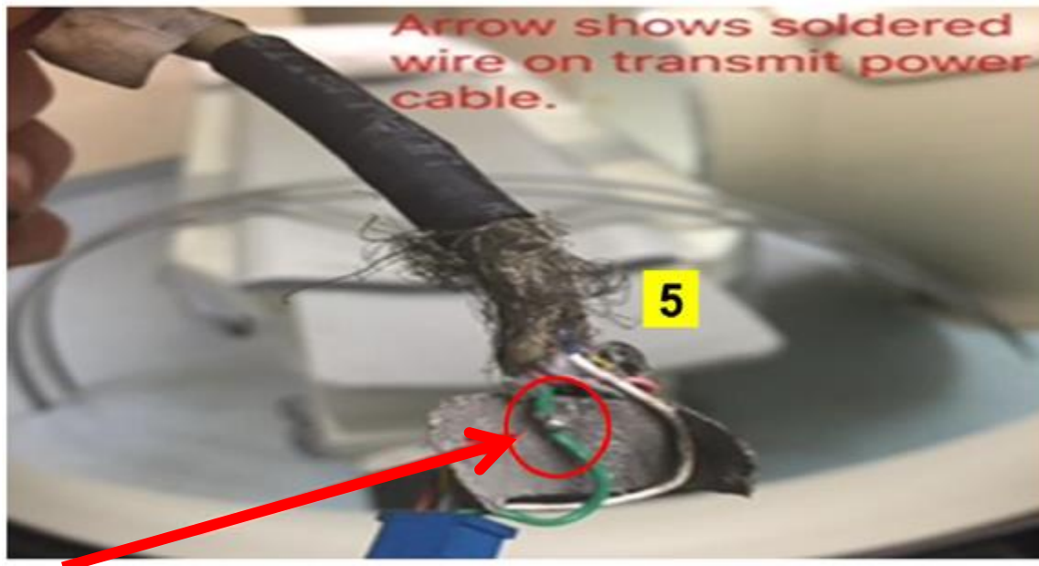
5. Transmit wire connection repaired previously and taped and visible and exposed at joint of green wire
